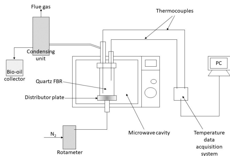
Figure 6. MAP setup used by Salema and Ani (Adapted from [68]).
